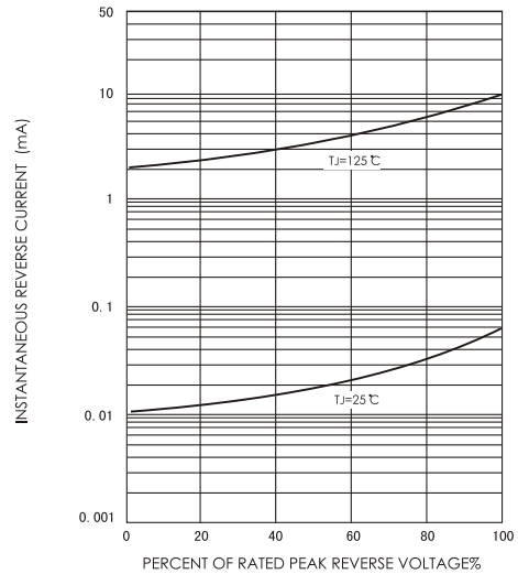
FIG.4-TYPICAL REVERSE CHARACTERISTICS
