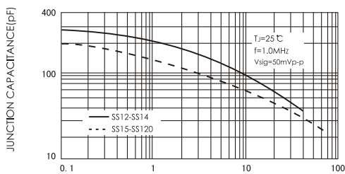
FIG.5-TYPICAL JUNCTION CAPACITANCE
